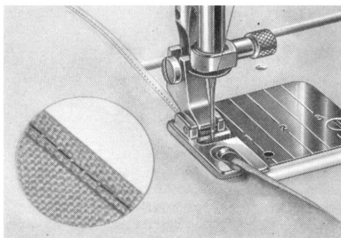
41 11 384. Straight stitch jointed hemmer, \frac{5}{64} " (2 mm).
