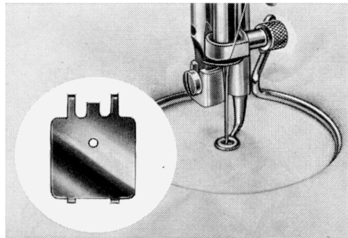
40 23 013 Presser foot, extra narrow, for straight stitching.
