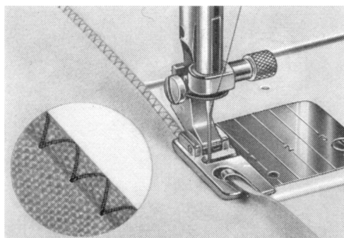
41 11 387. Jointed hemmer for rolled seams, \frac{5}{64} " (2 mm), zig-zag. Suitable for thin material.
